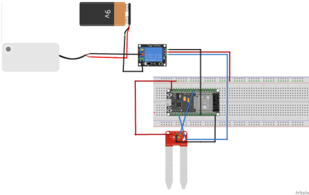
Figure: Fritzing schematic drawing of hardware setup
