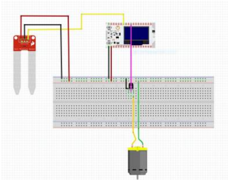
Fig4: Shows the Hardware connections of the experiment.
