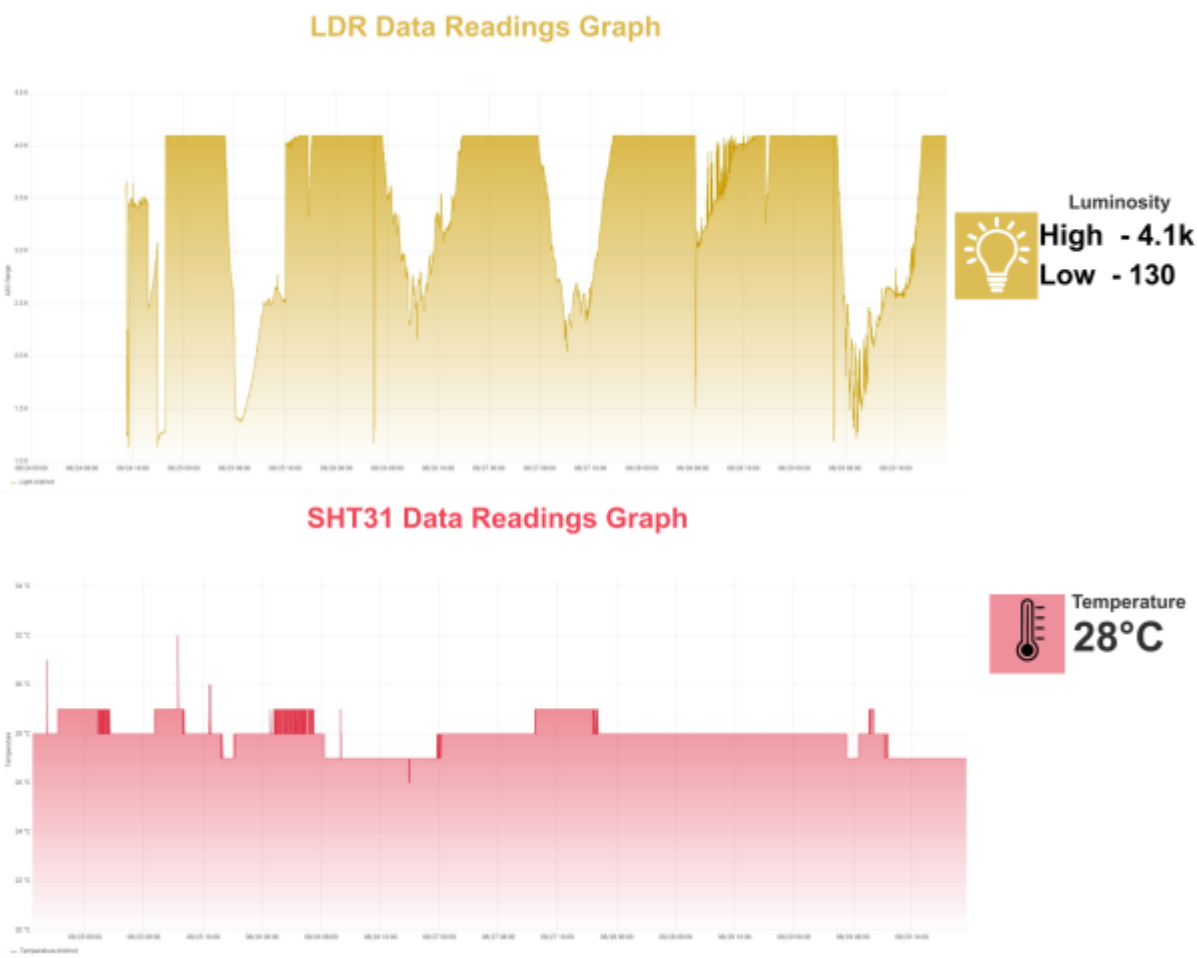
Fig. 16 Measurement results of the SHT-31 and LDR sensors visualized in Grafana
