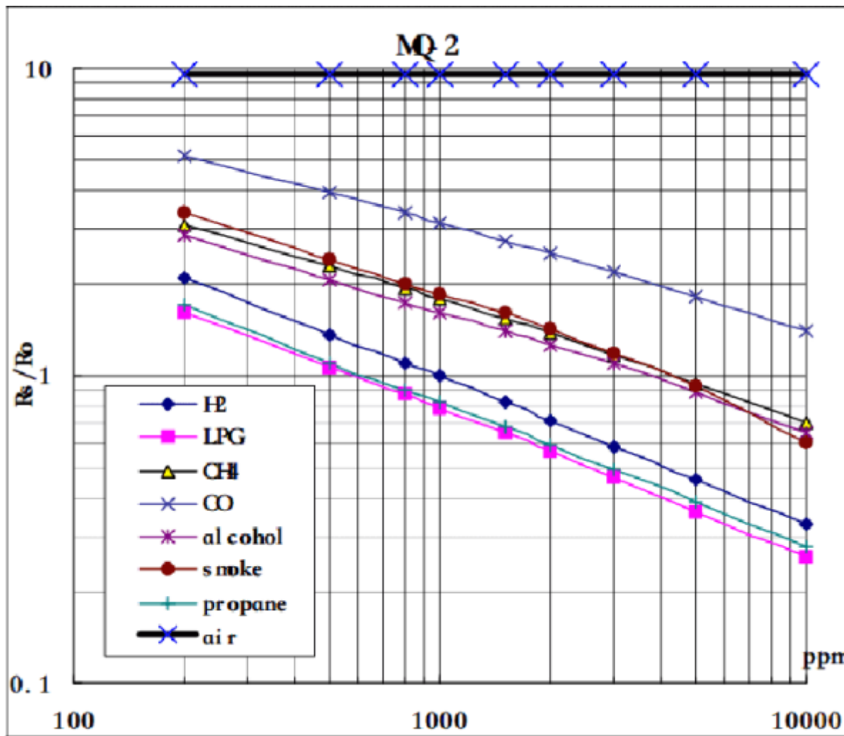
Figure 2.3 MQ2 Sensitivity characteristics. Source: https://www.mouser.com/datasheet/2/321/605-00008-MQ-2-Datasheet-370464.pdf }
