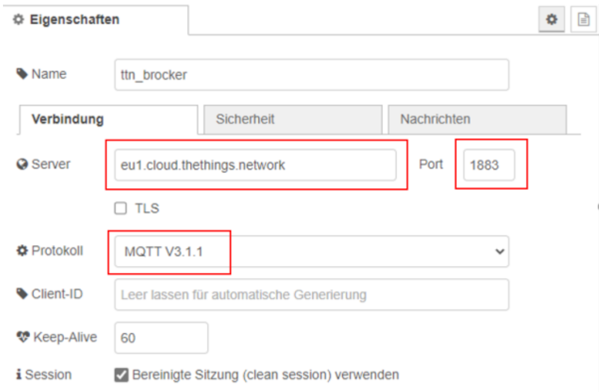
Figure 37: connection parameters
