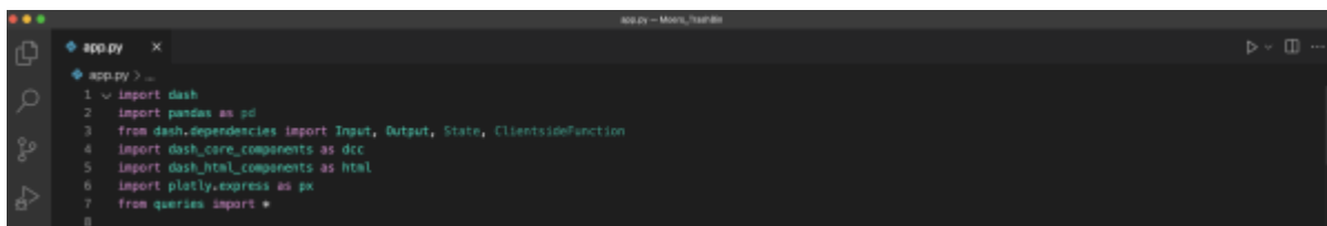
Figure 49: Import Libraries
