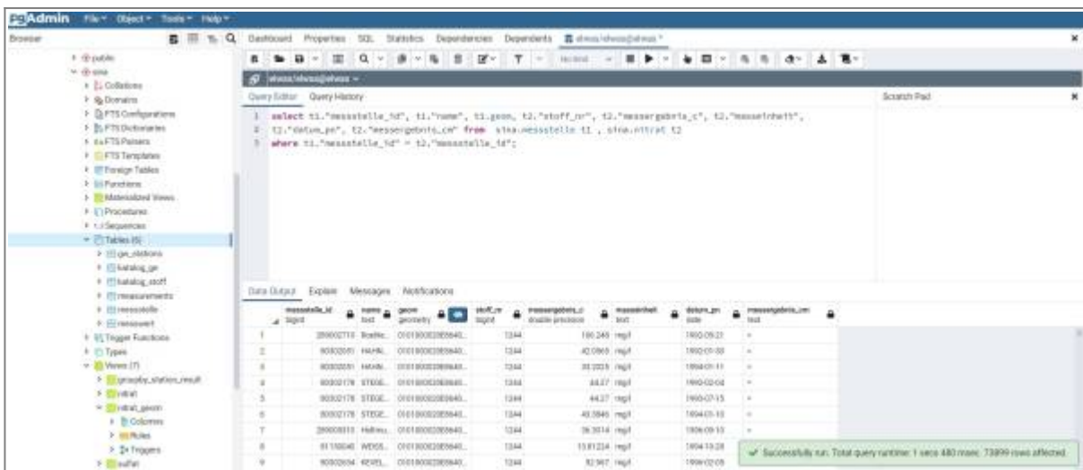
Image 13- Merge tables
