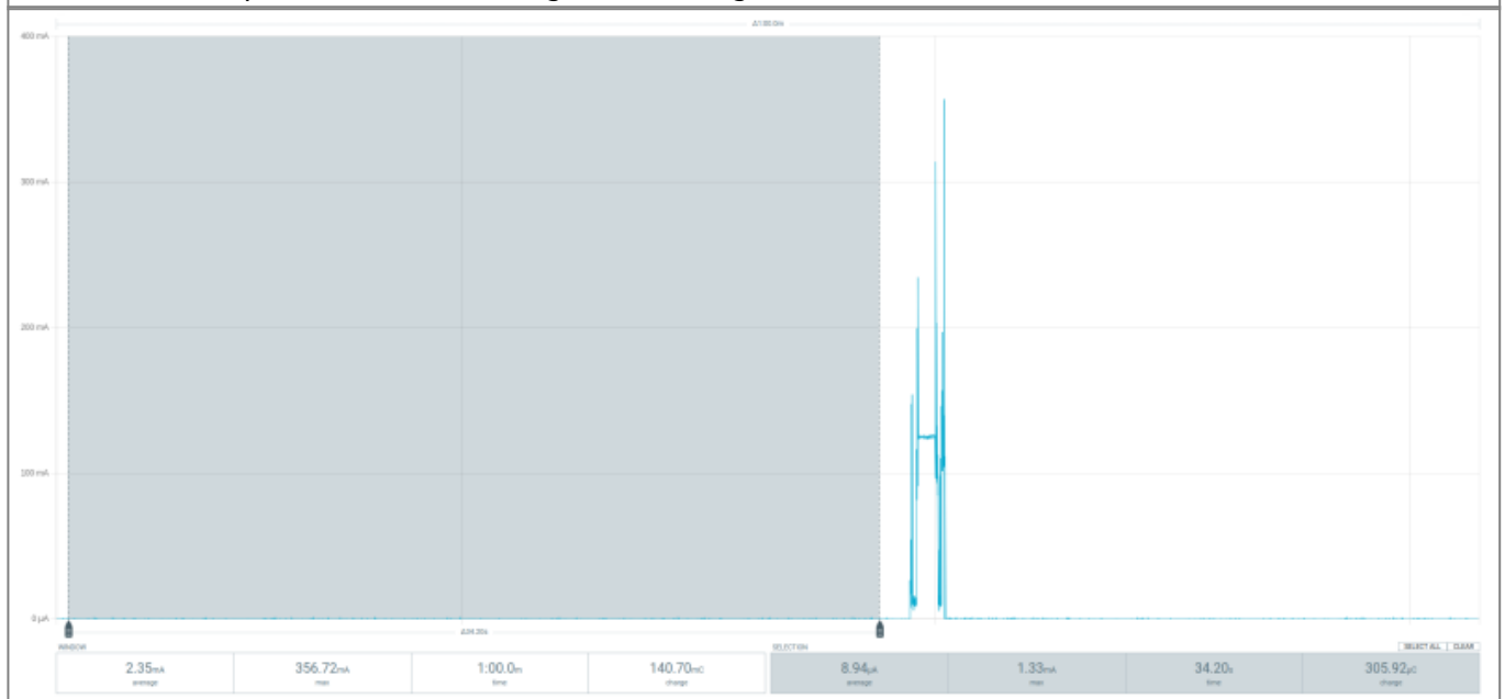
Current consumption while in deepsleep is around 9µA
