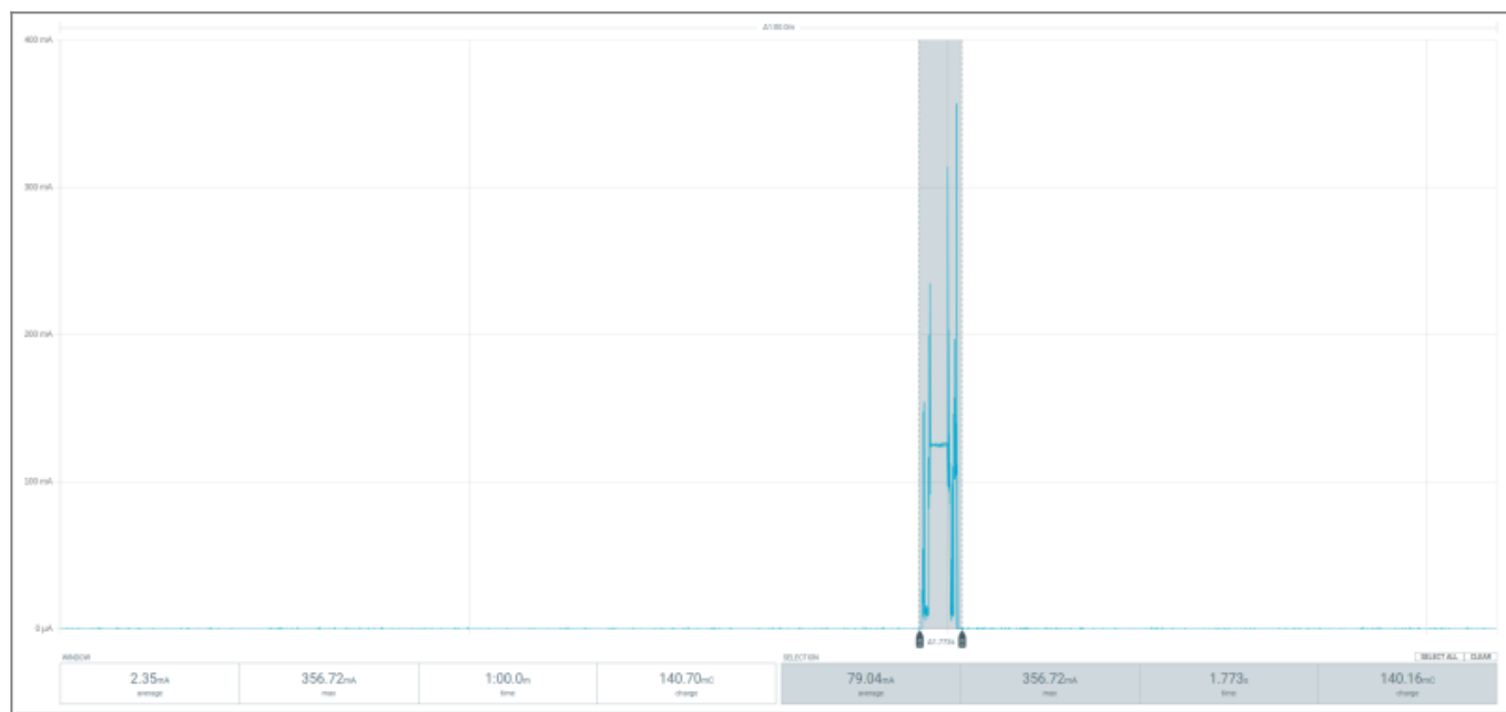
Current consumption while measuring and sending is around 80mA for 1.8 seconds
