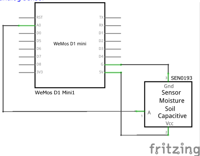
Fig. 1: Wiring of the analog sensor
