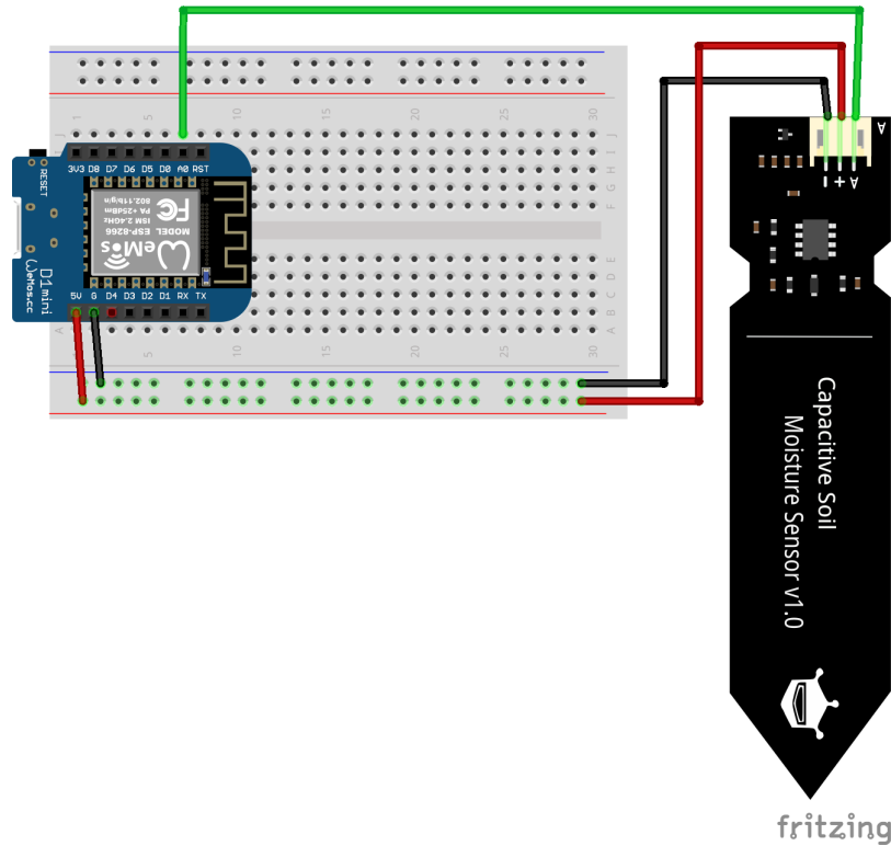
Fig. 1: Wiring of the analog sensor
