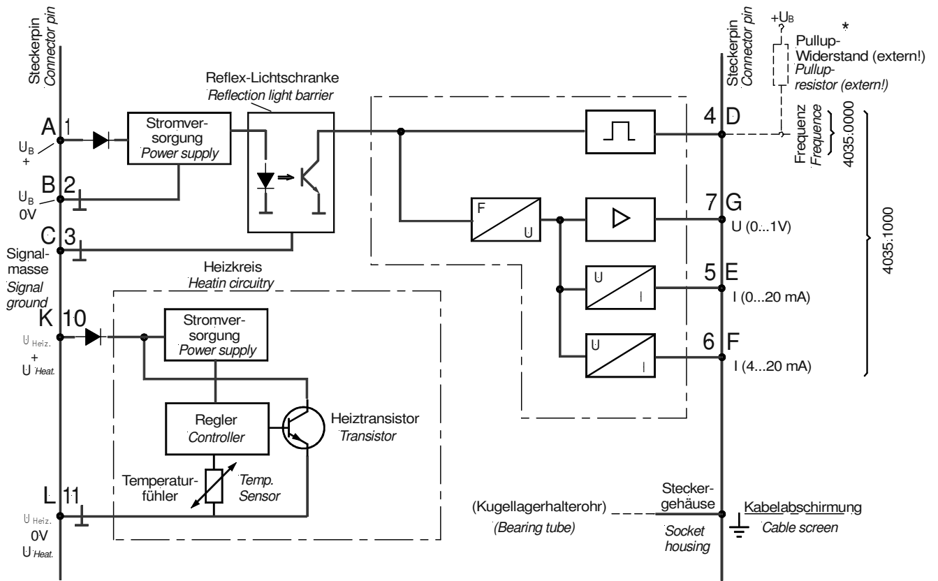
FIG. 3: BLOCK DIAGRAM / CONNECTION PLAN
