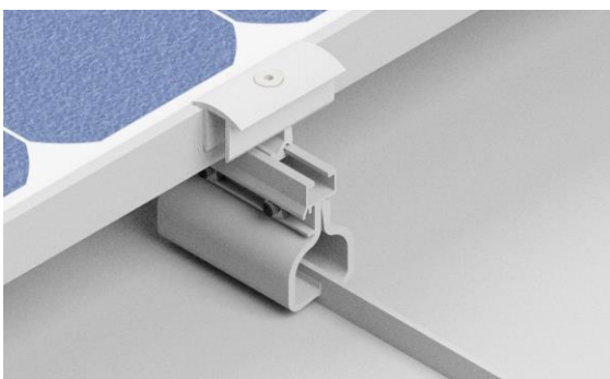
Figure 105: Direct assembly
