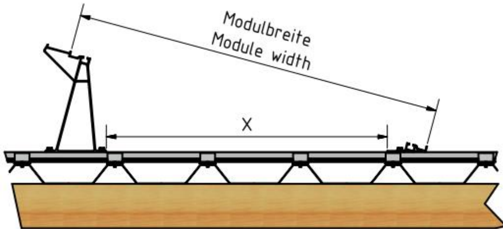
Figure 81: Distance AeroFix 15-S supports
