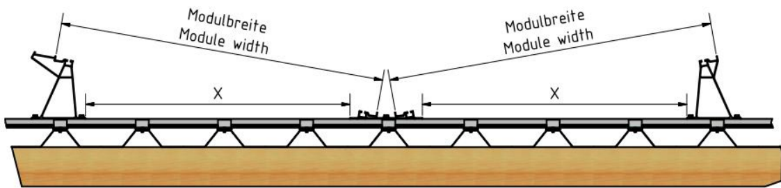
Figure 83: Distance AeroFix 10-EW supports
