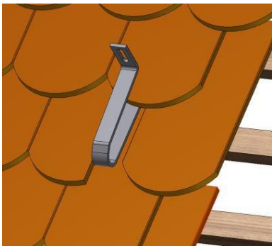
Figure 26: Depression for "Biber S"
