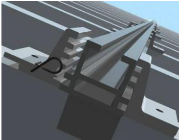
Figure 62: Insert the carrier rail
