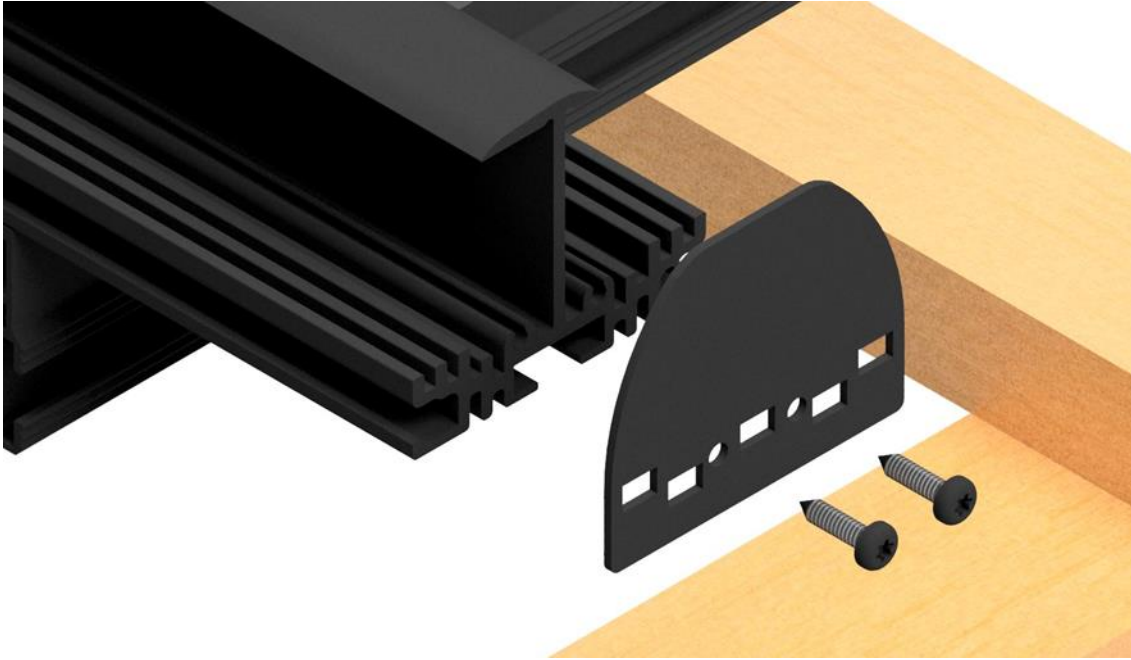
Figure 152: Side plate
