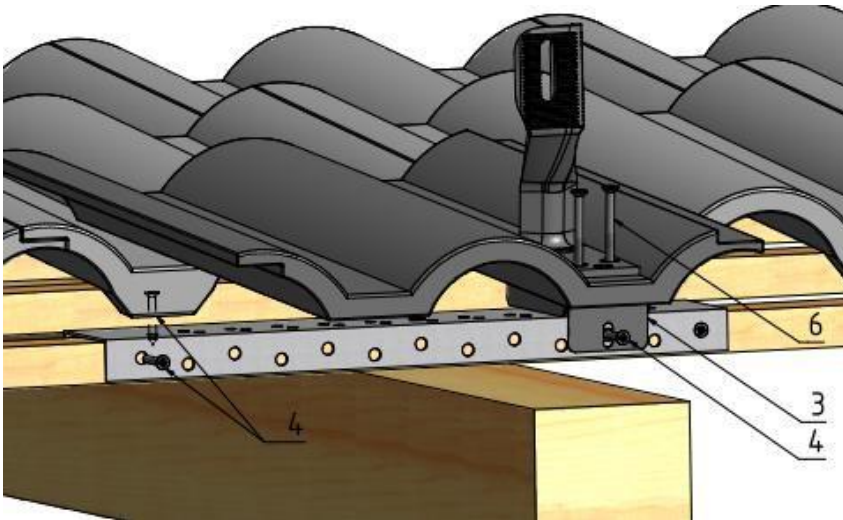
Figure 41: Connecting sheet metal roof tiles with batten rail
