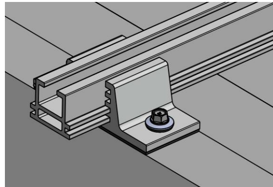
Figure 70: Trapezoidal clamp screwed
