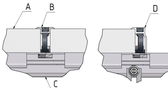
Figure 112: Assembled clamps (sectional view)
