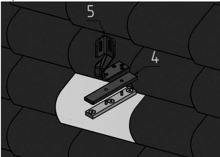
Figure 47: Cover cap and roof hook
