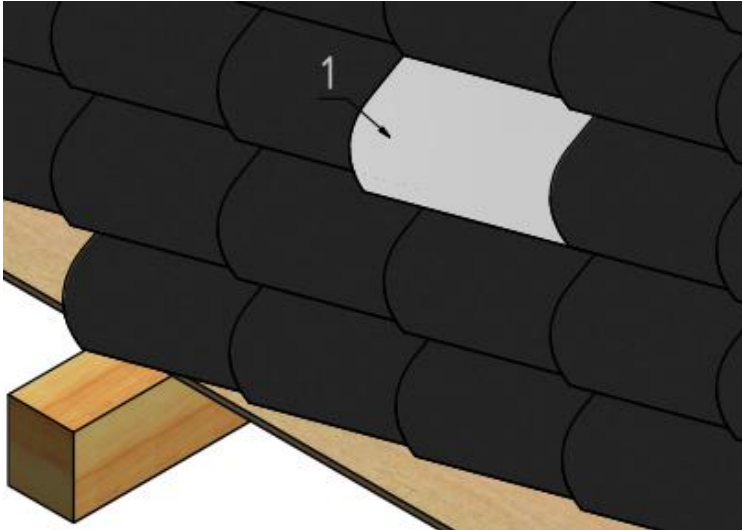
Figure 45: Insert the metal plate (slate roof only)
