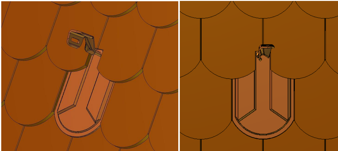
Figure 43: "Mammut Form S+" plain tile dual roofing
