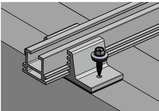
Figure 101: Apply the screw
