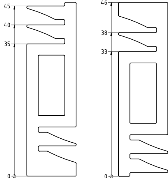
Figure 116: EC adapter frame heights
