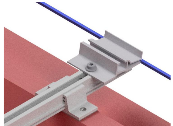
Figure 80: Mounted Bottom Support
