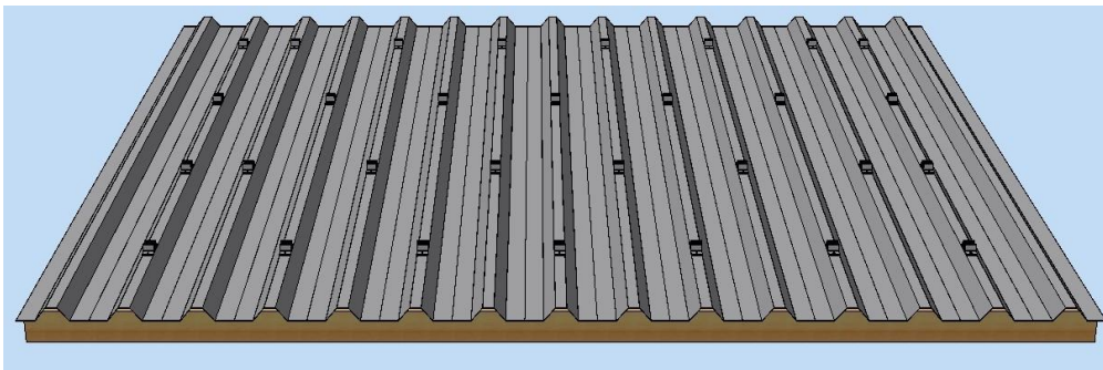
Figure 61: Distribute the clamps according to the instructions
