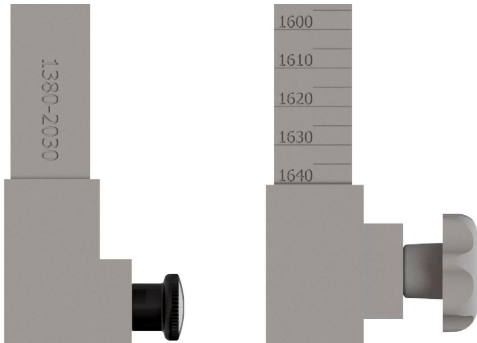
Figure 136: Adjusting the assembly jig
