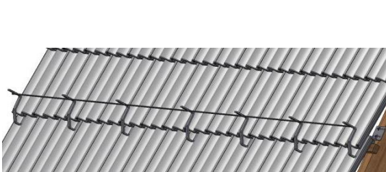
Figure 8: Fitted roof hook
