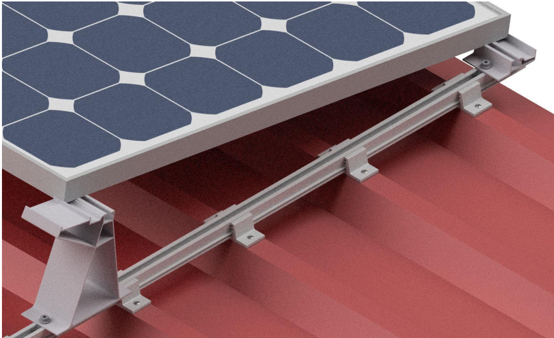
Figure 86: Insert the module in the Bottom Support and Top Support
