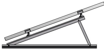
Figure 129: Vertically mounted modules with module carrier rail
