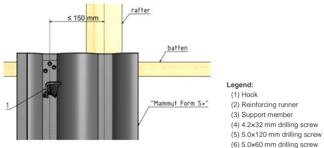
Figure 39: "Mammut Form S+" roof hook
