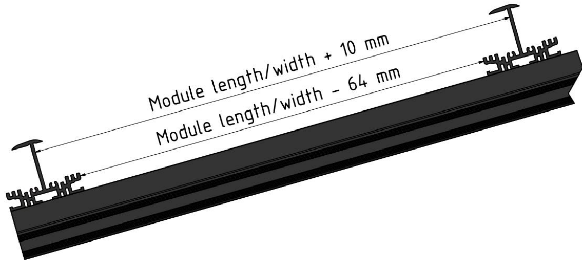
Figure 135: Insertion rails distance: Module length / -width + 10 mm, or module length / width - 64 mm
