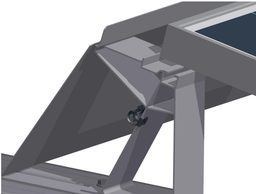
Figure 118: cable clip 90° on support profile
