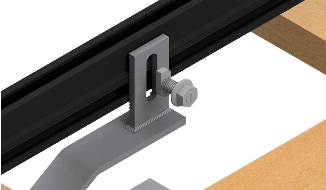
Figure 133: roof connector rail assembly
