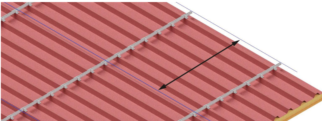
Figure 78: Mark the position of the Bottom Support in the grid spacing
