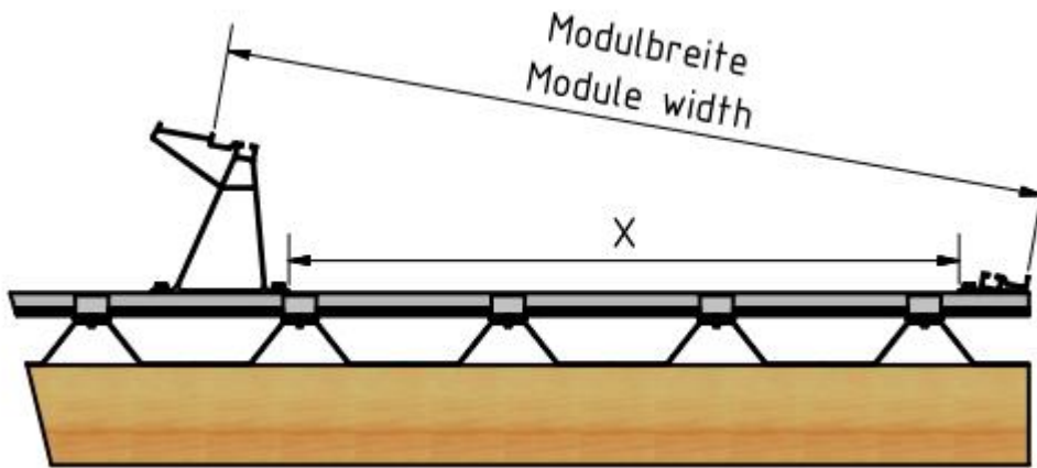
Figure 82: Distance AeroFix 10-S supports
