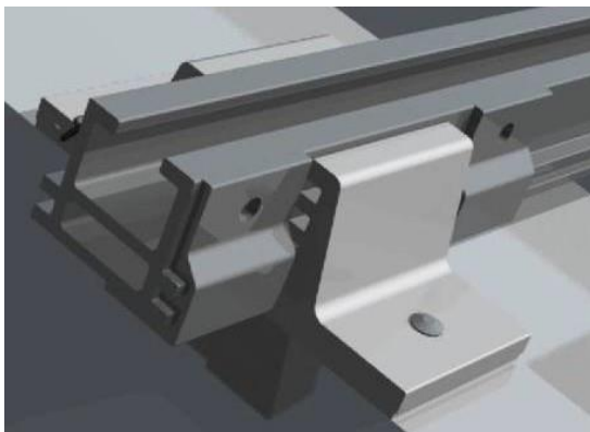
Figure 71: Insert transverse securing clamps
