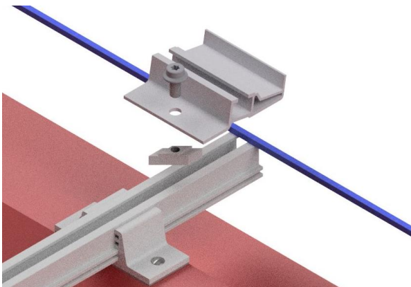
Figure 79: Bottom Support with screw and rhombus nut
