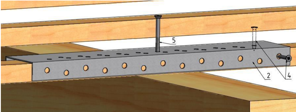
Figure 40: Fastening the batten rail
