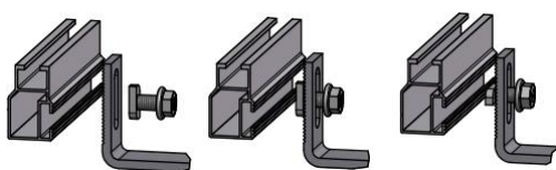
Figure 110: Fitting carrier rails
