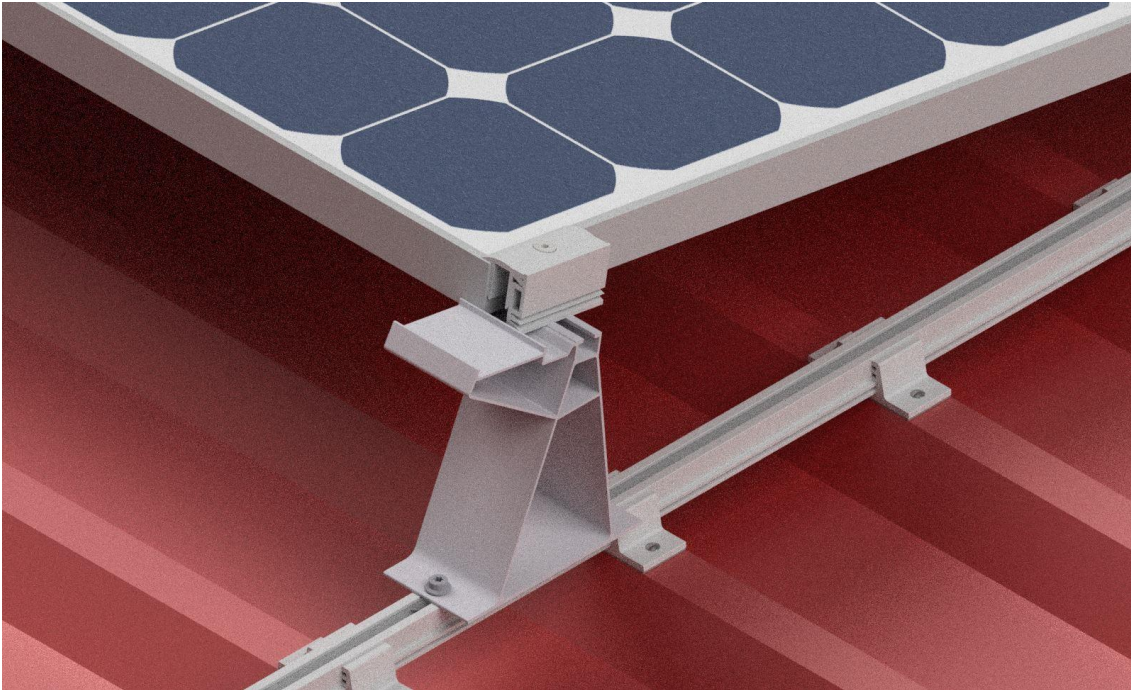
Figure 88: Module at the stop of the Top Support and clamped
