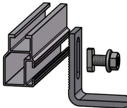
Figure 109: Mounting carrier rails
