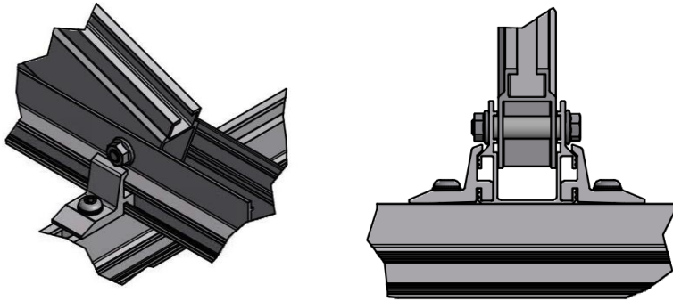
Figure 128: Two-layer fixation (two-layer connector)
