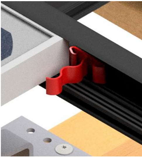
Figure 149: Attach spacer
