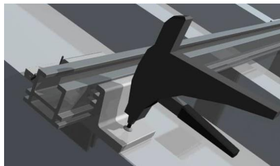
Figure 68: Riveting using a standard rivet head
