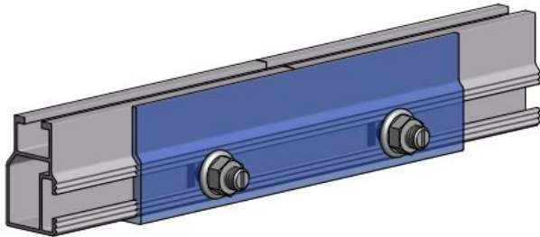
Figure 111: Butt connectors for type TF50 carrier rails
