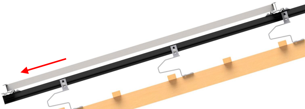
Figure 148: Slide module into position
