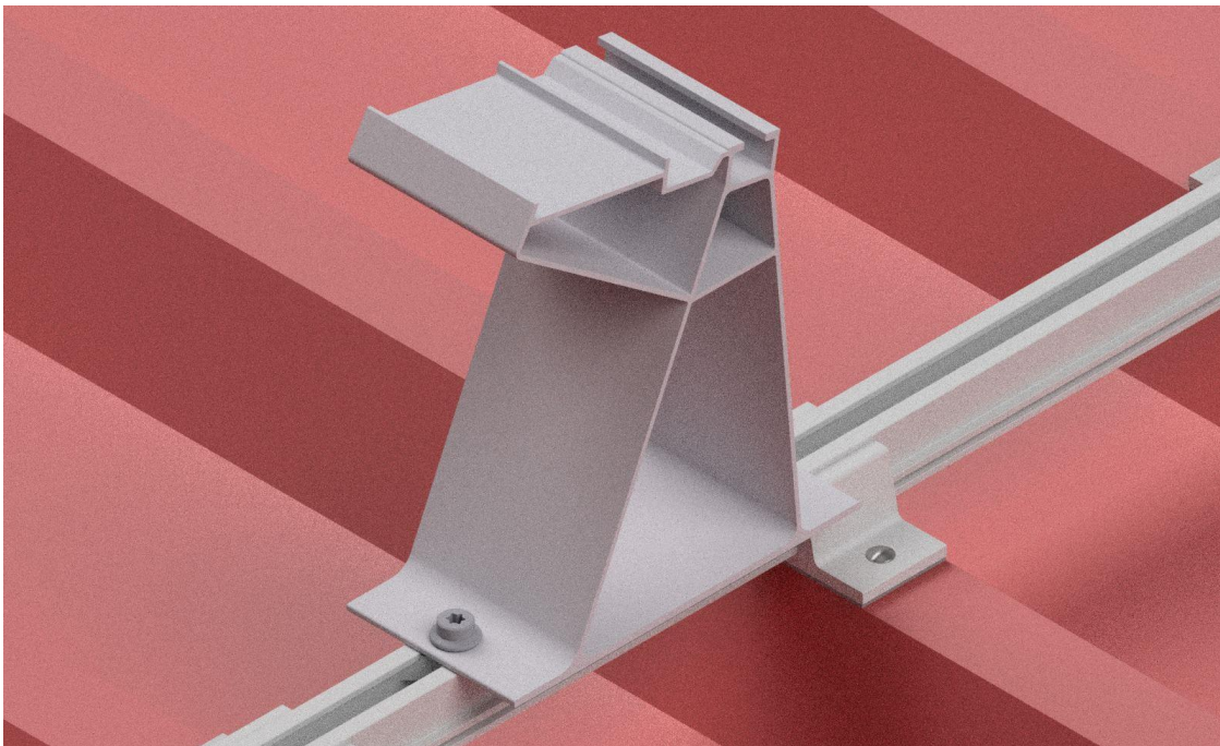
Figure 85: Mounted Top Support
