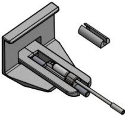
Figure 160: Tensioning piece and adapter
