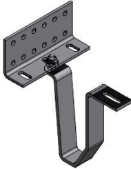
Figure 21: “Vario S+” roof hook
