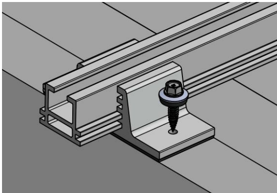
Figure 69: Apply the screw
