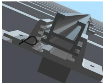
Figure 63: Align the carrier rail
