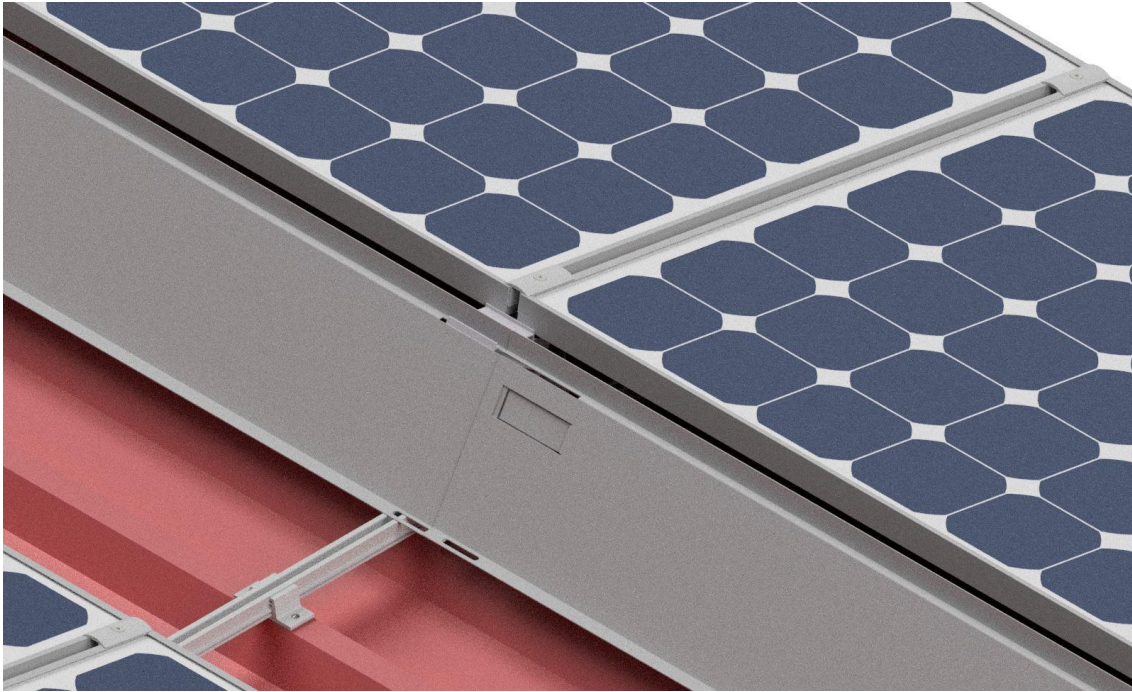
Figure 91: Insert wind plate
