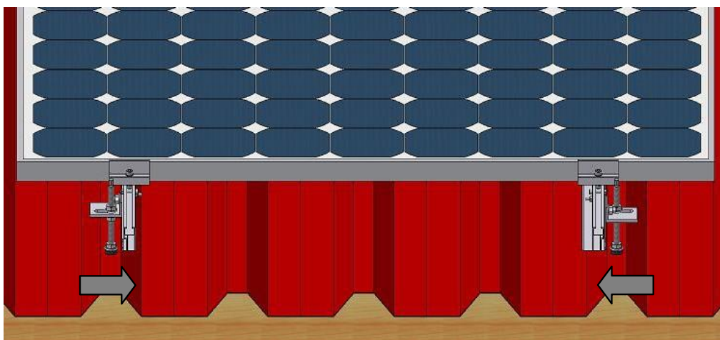
Figure 53: Mounted hanger bolt with "universal connector"
