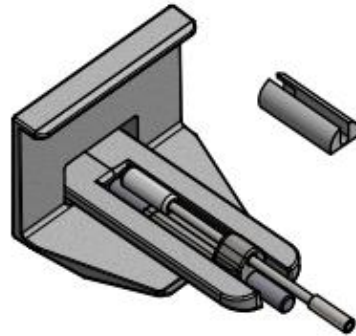
Figure 161: Disconnect the cable from the tensioning piece
