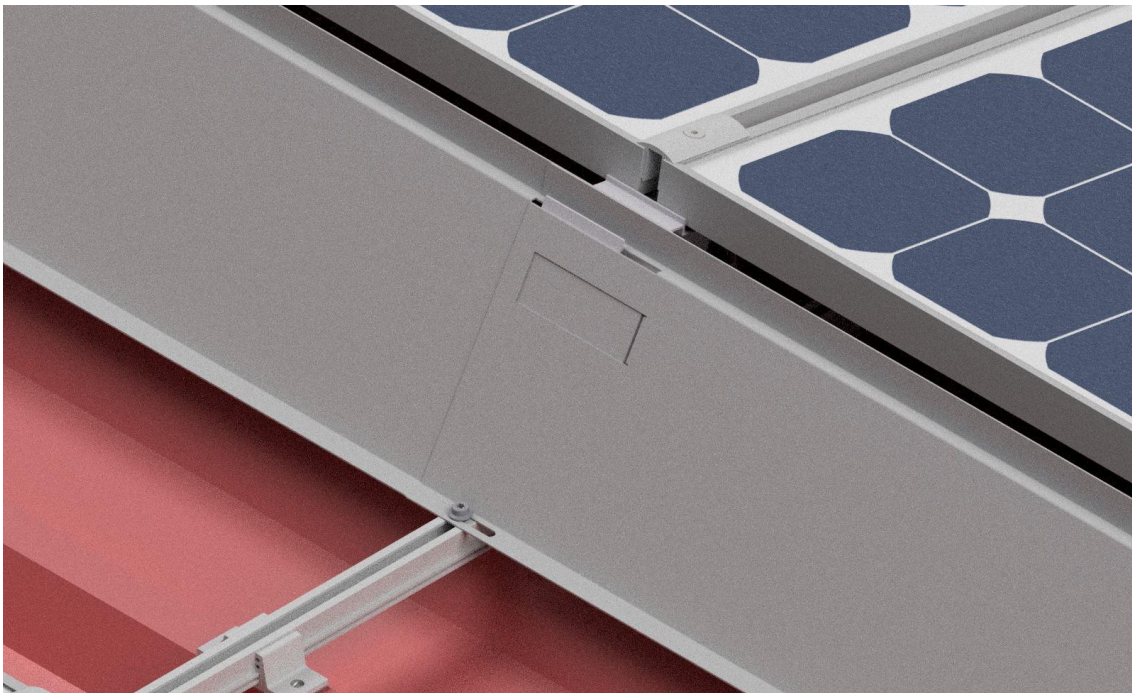
Figure 92: Fixed wind plates within the row
