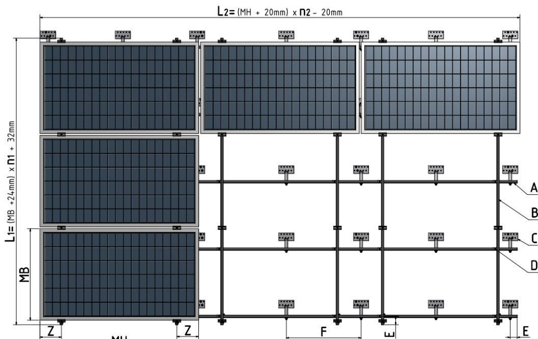
Figure 119: Roof hook connecting rails and carrier rails as a unit
