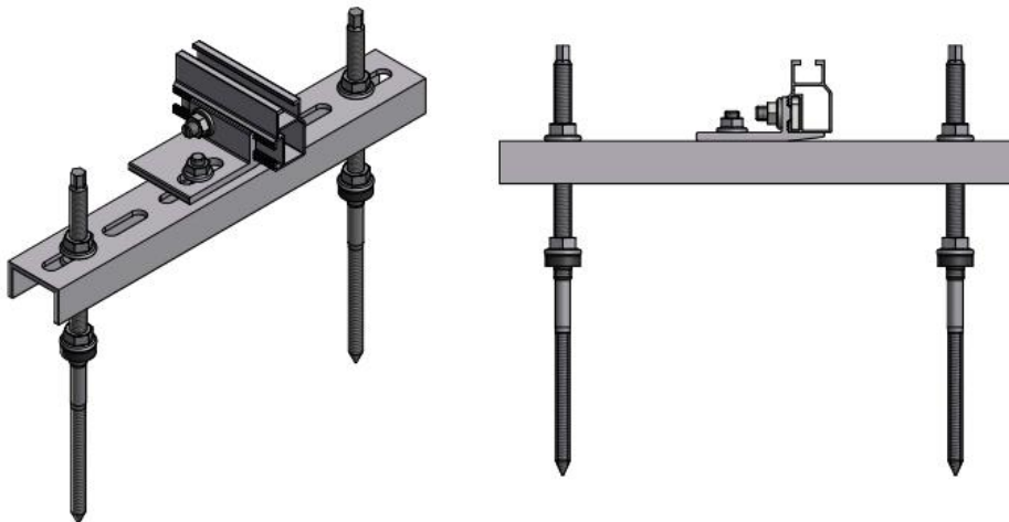
Figure 56: Mounting plate Duo with universal connector
