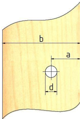
Figure 167: Defining the distance to the edge of rafters
