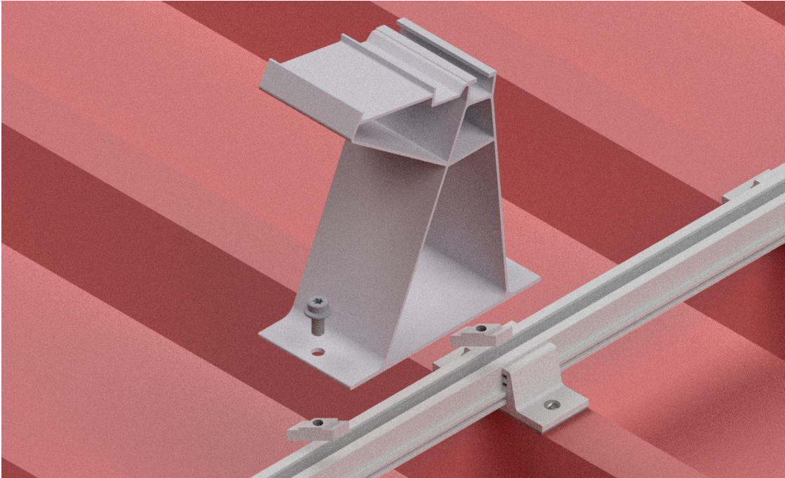
Figure 84: Fasten Top Support with two screws and rhombus nuts
