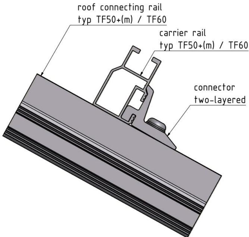
Figure 120: Cross section of a two-layer system structure
