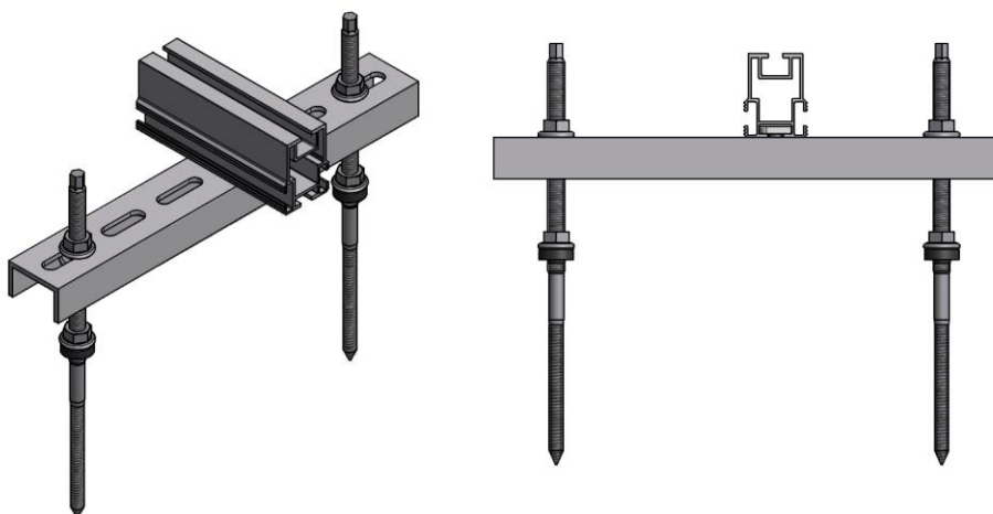
Figure 57: Mounting plate duo with connecting element RH-profile
