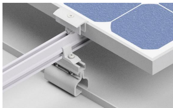
Figure 106: with support rail and 2-layer connector
