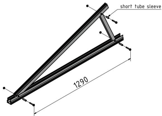
Figure 124: Assembling Delta supports at the base rails
