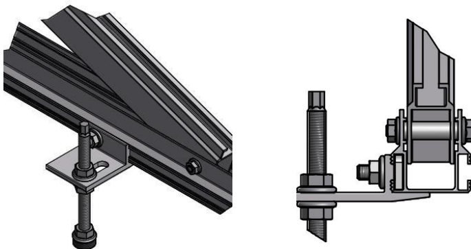
Figure 127: Fixation by universal connector
