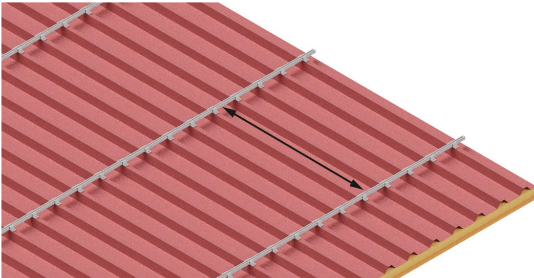
Figure 77: Gap = Module length + 20 mm
