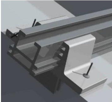
Figure 99: Inserting blind rivets
