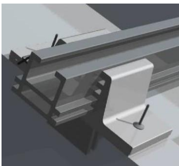
Figure 67: Inserting blind rivets
