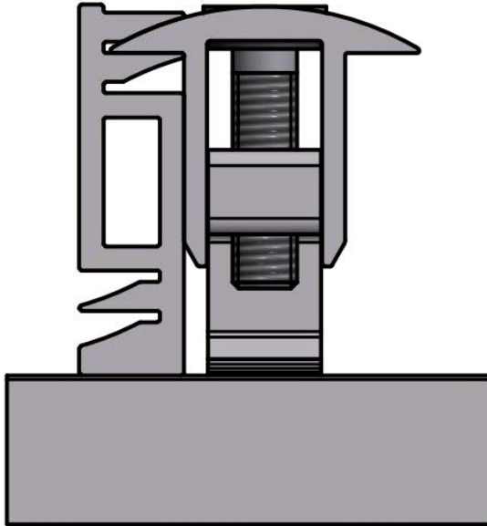
Figure 115: EC adapter with middle clamp G4
