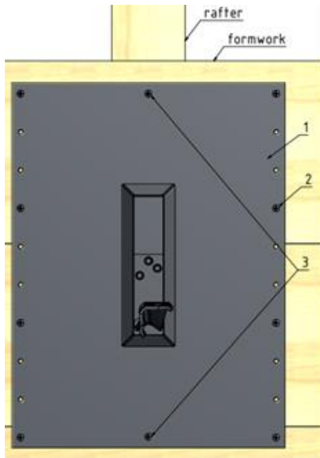
Figure 42: "Mammut Form S+ Bitumen"
