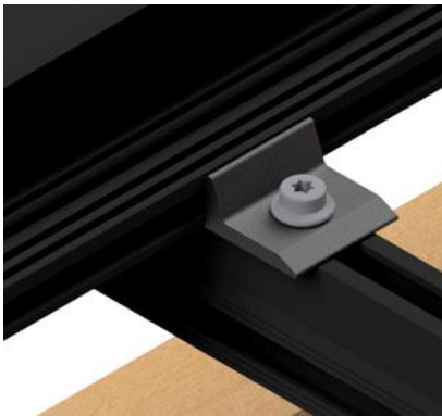
Figure 140: Two-layer connector
