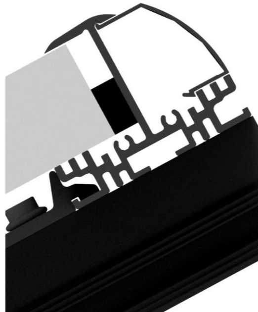
Figure 156: Mounted end cover at the top
