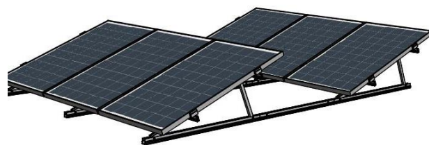
Figure 123: Delta support with continuous base rail
