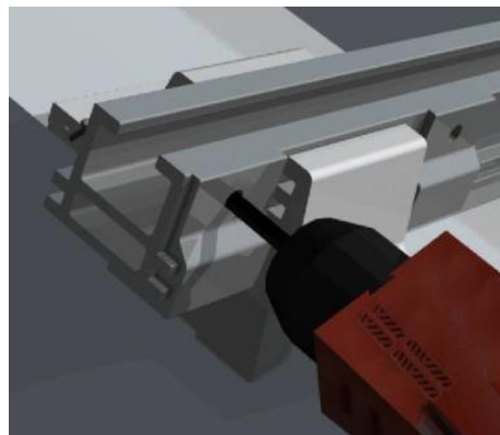
Figure 72: Drilling transverse securing clamps
