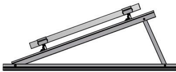
Figure 130: Horizontally mounted modules with module carrier profiles
