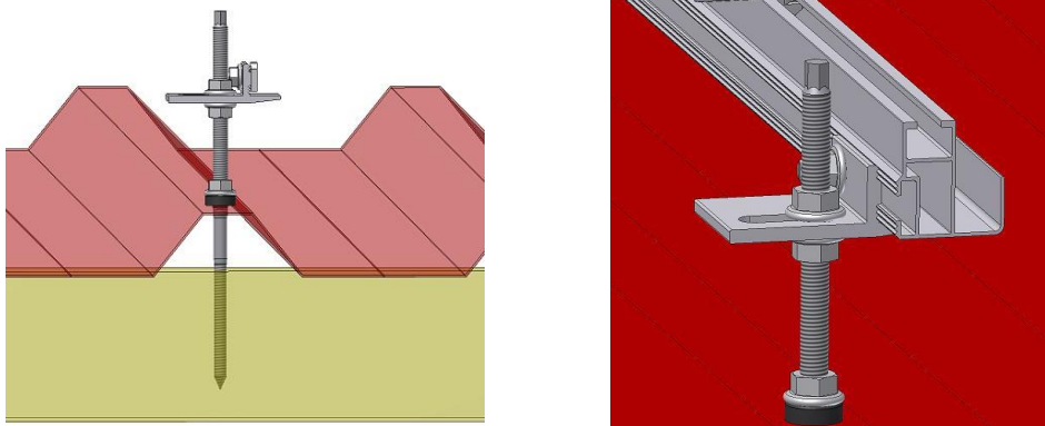
Figure 51: Correctly fitted hanger bolt with universal connector
