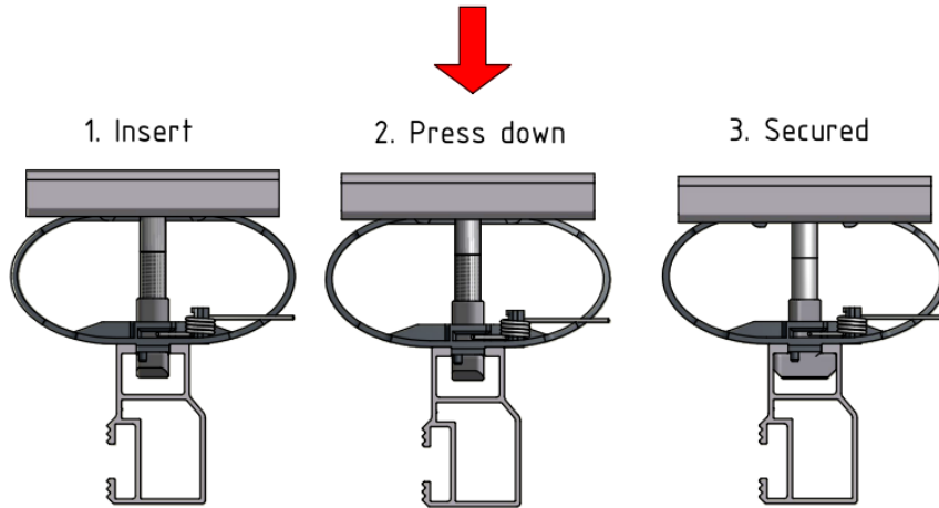
Figure 113: Inserting middle clamps G3
