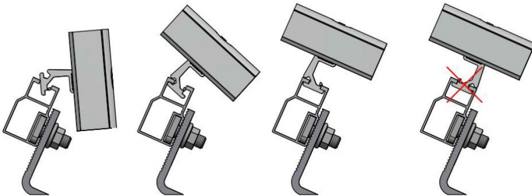
Figure 114: Inserting middle clamps G4
