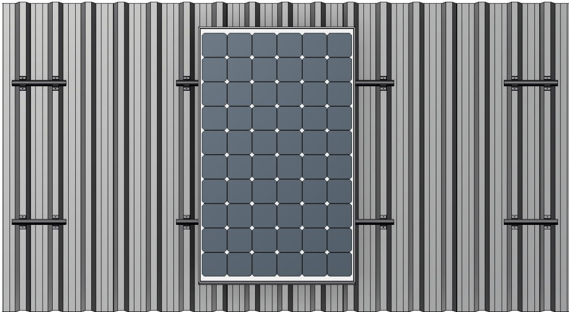
Figure 103: Aligning PV modules
