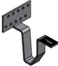
Figure 15: "Mammut S+" roof hook
